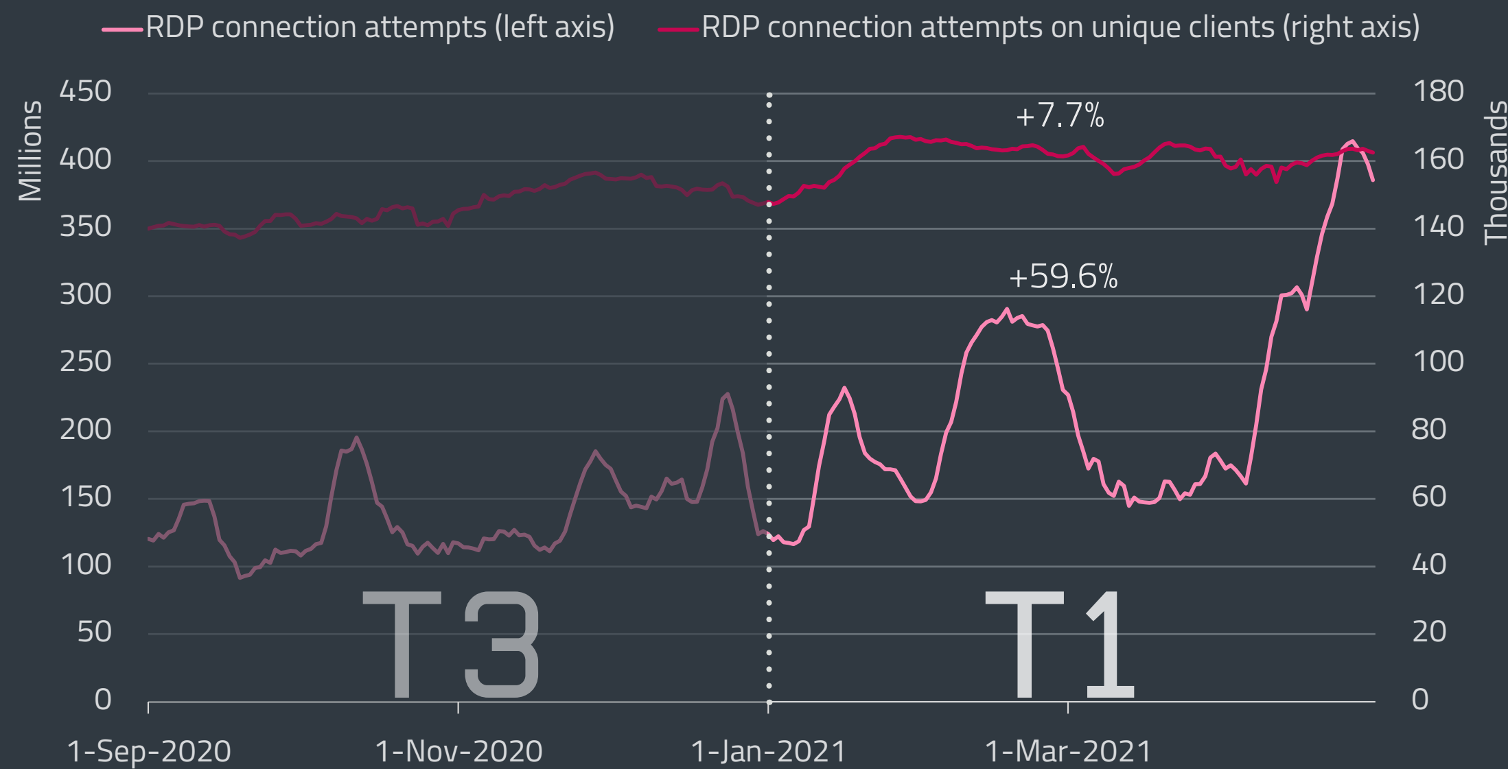
Trends of RDP connection attempts and unique clients in T3 2020 – T1 2021, seven-day moving average
