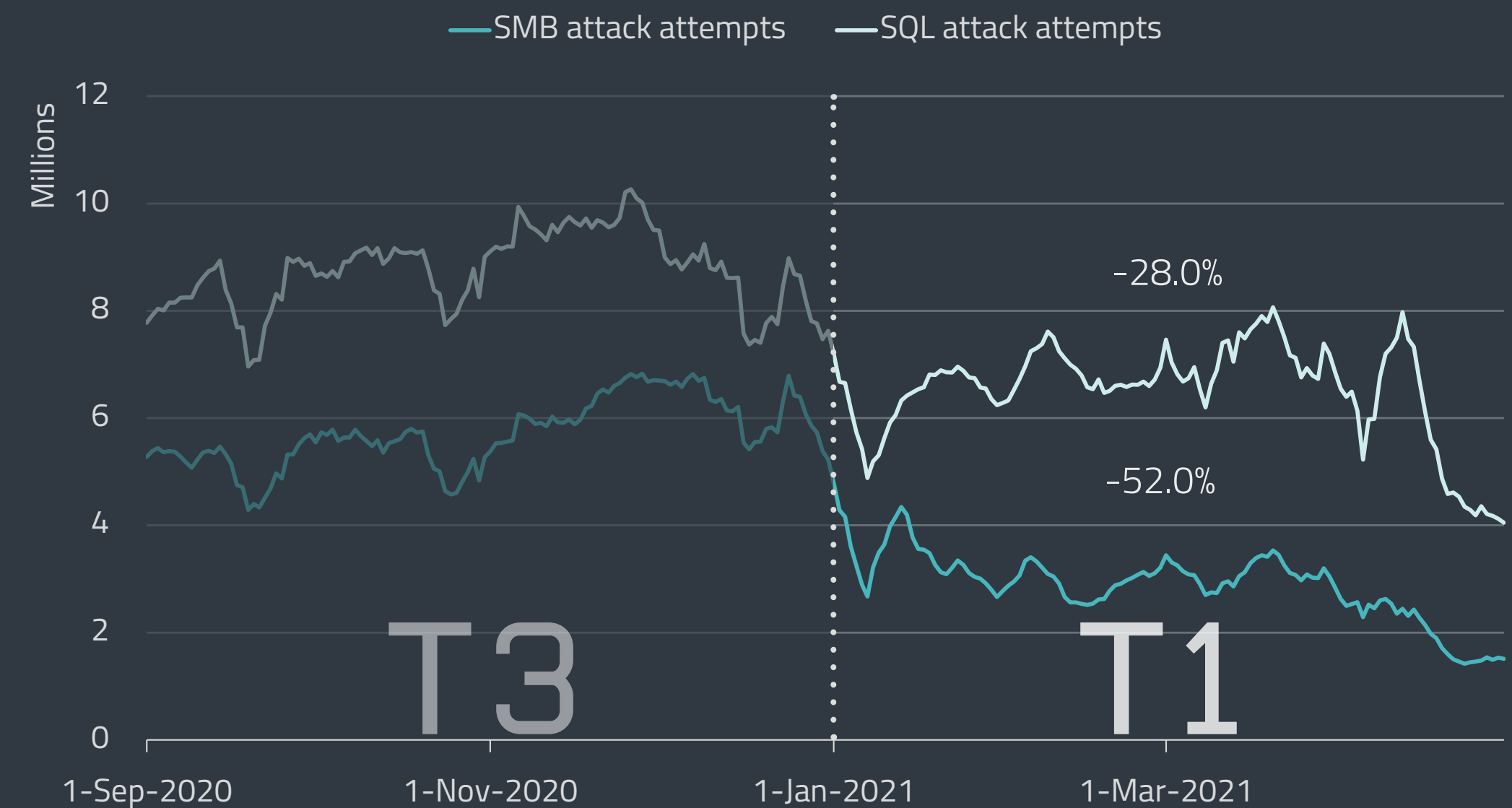
Trends of SMB and SQL connection attempts in T3 2020 – T1 2021, seven-day moving average
