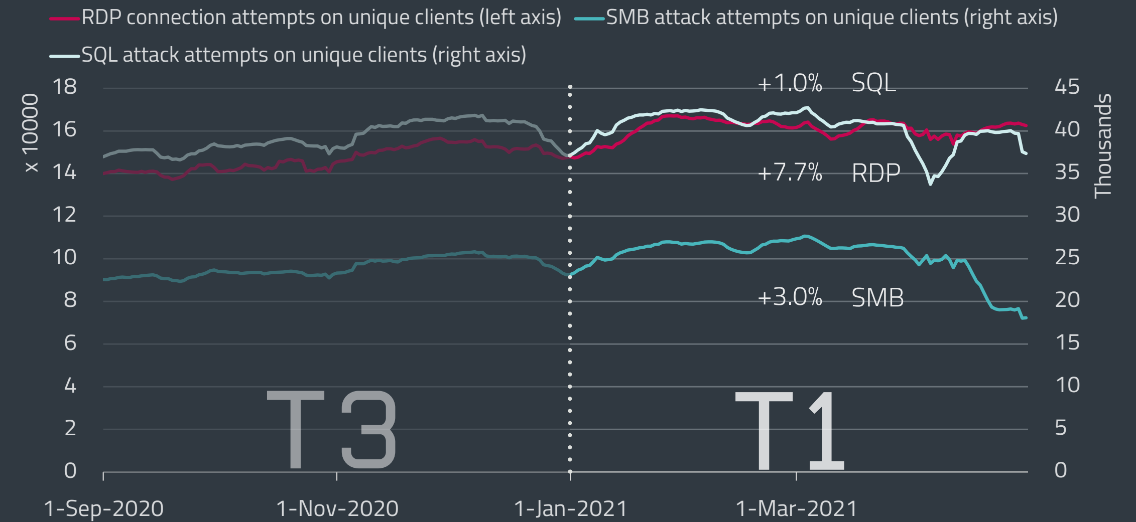
Trends of RDP, SMB and SQL connection attempts on unique clients in T3 2020 – T1 2021, seven-day moving average
