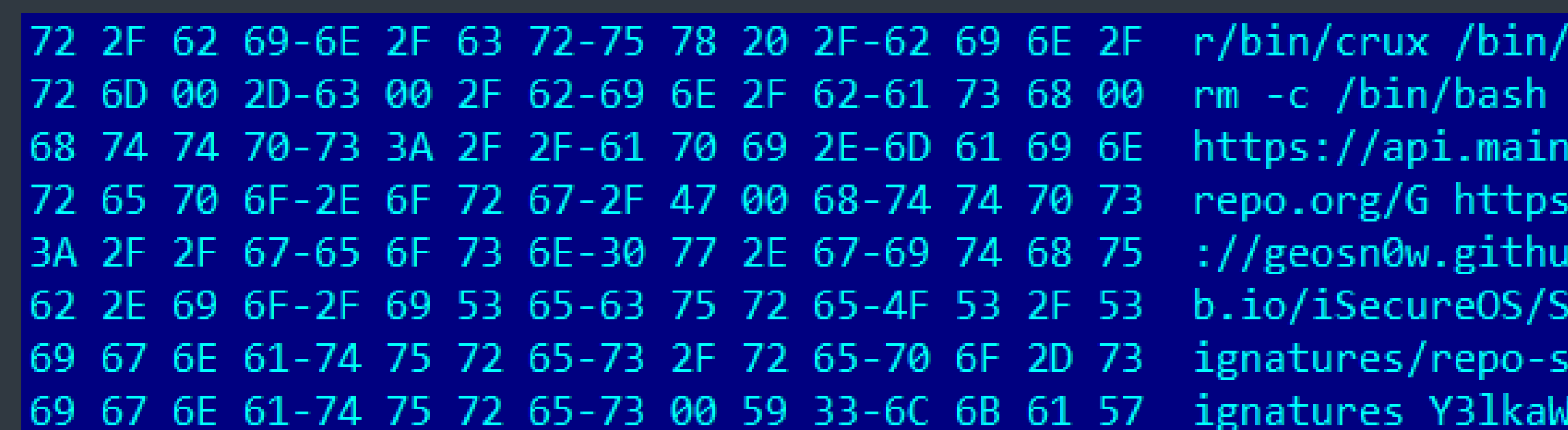
Decrypted strings of newer version of iOS/Spy.Postlo.A
